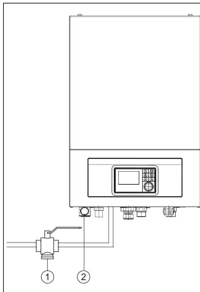
Afb. 6 Binnenunit IDU Monoblock E
